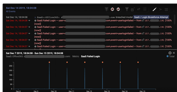
Figure 30: A graph illustrating the repeated login attempts
